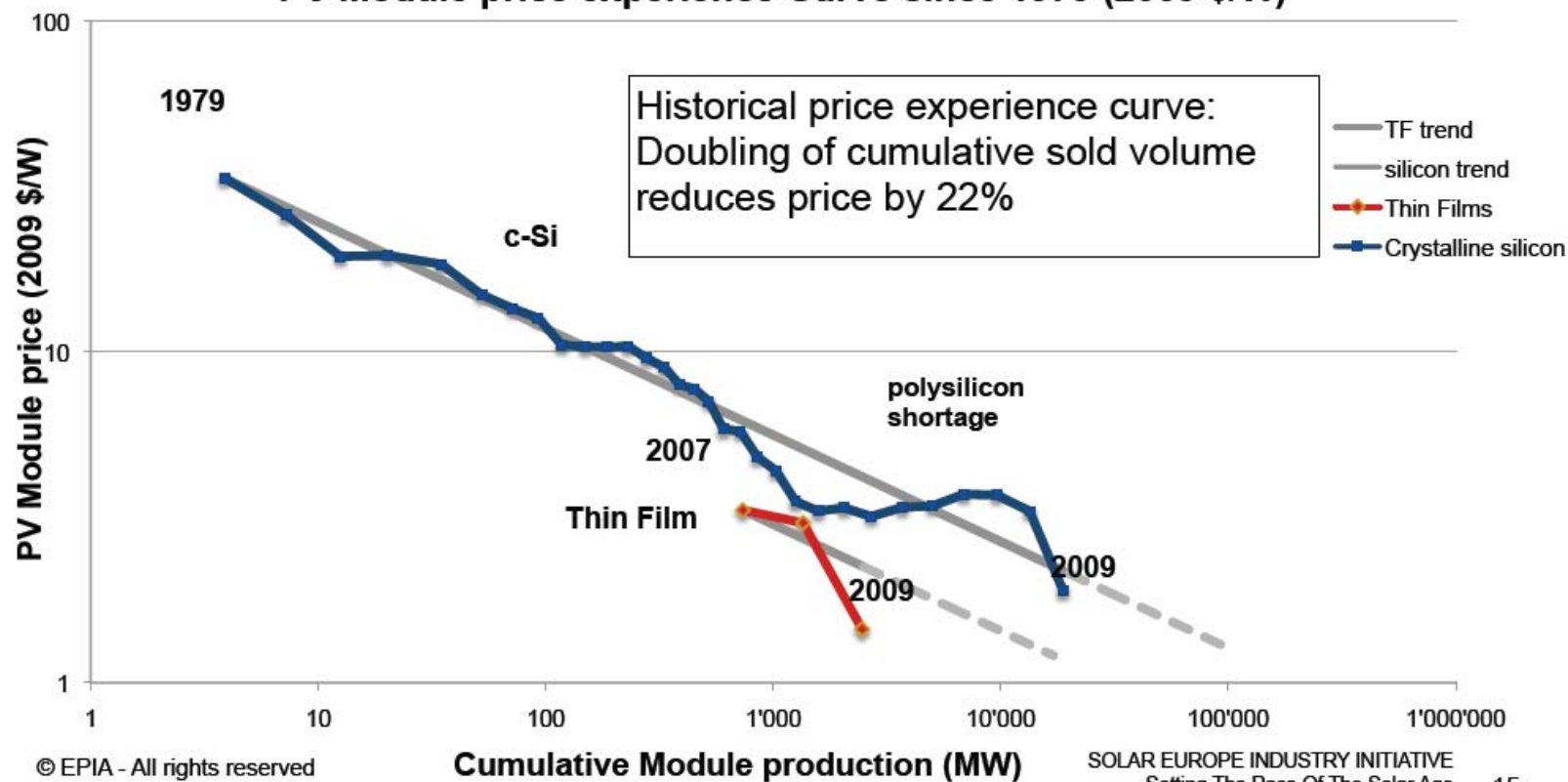
PV Module price experience Curve since 1979 (2009 $/W)
